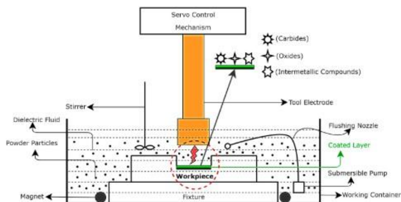
1.1 Typical arrangement of PMEDM system
